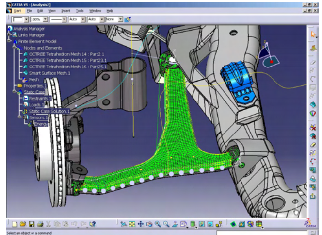
Screen capture of CATIA - FEM and Structural Analysis
