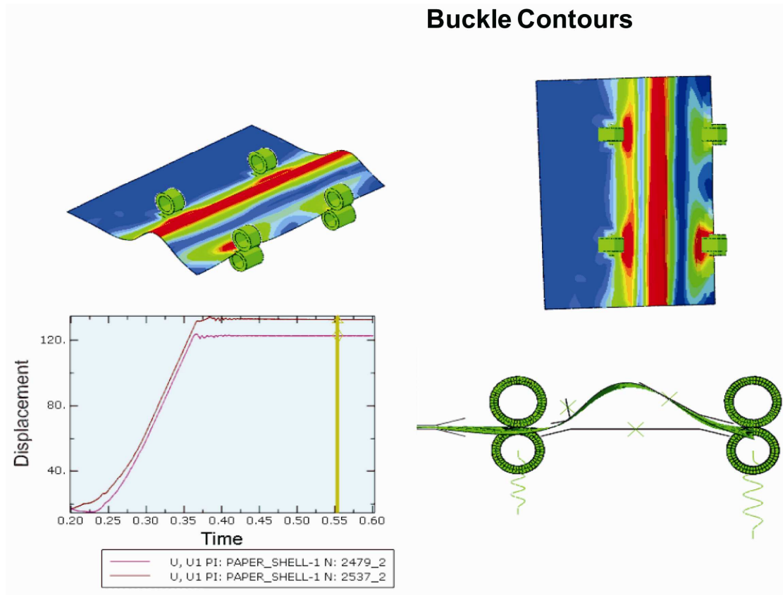
Figure 2. Results from 3D paper buckling contour analysis using Abaqus FEA. When paper flow and roller nip forces are imperfectly balanced, a buckle of paper can rise up, filling the paper path and resulting in paper slip and/or stubbing (paper jam). HCL's engineers use such data to examine the relationship between such forces in different printer designs so they can make modifications that resulting in optimum paper flow.
