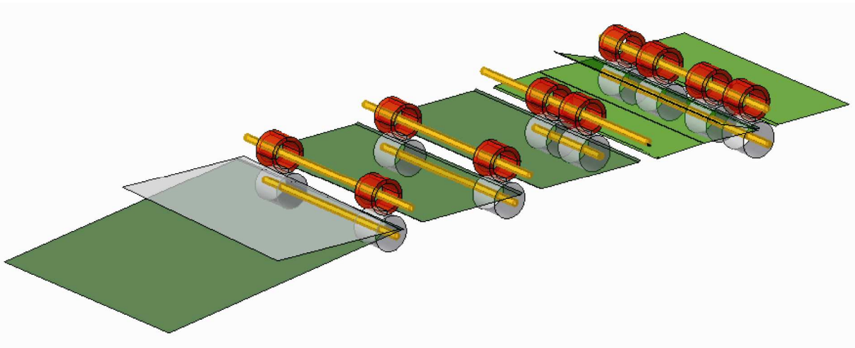
Figure 1. 3D CAD model of a typical printer paper flow path. The paper is pulled into the printer ('nipped') between a rotating upper rubber roller (the drive) and a stationary, spring-loaded lower plastic roller (the driven, or idler). During the printing process the paper is conveyed through a series of these rollers, with baffles and stationary guides (not shown) directing its path.
